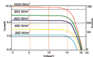
I-V-CURVE
